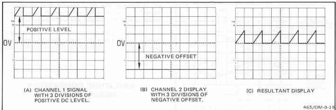
Fig. 16. Algebraic addition.
