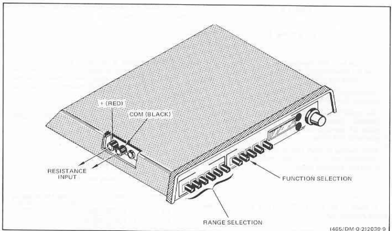
Fig. 8. Resistance.
