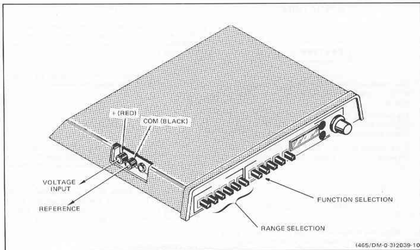
Fig. 9. Volts.
