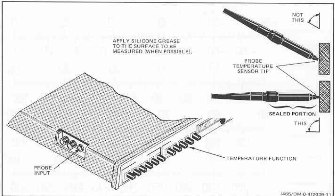
Fig. 10. Temperature.
