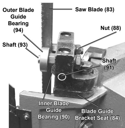
Figure Q: Lower Blade Guide Assembly
