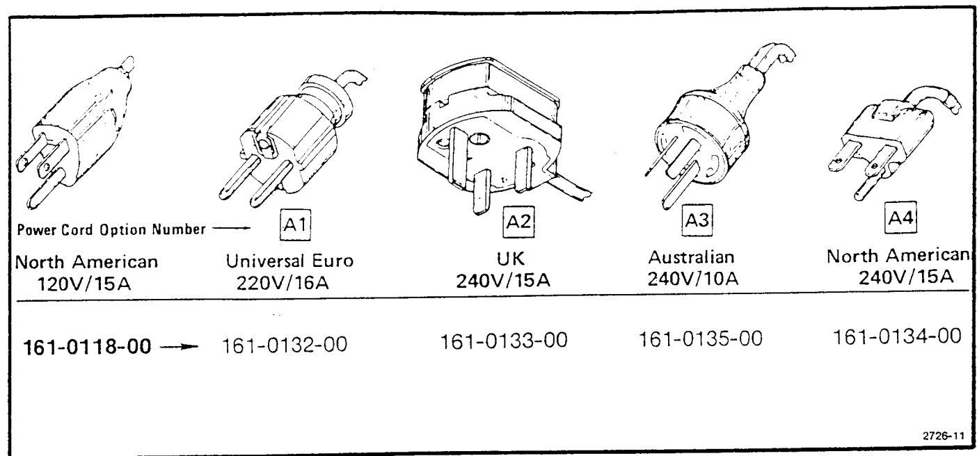
Fig. 1-2. International power cord and plug configuration for the 492.
