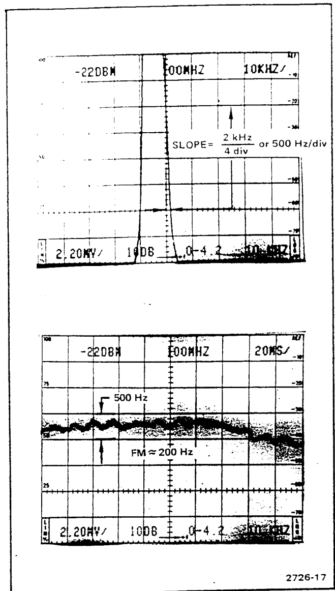
Fig. 3-7. Display that illustrates how to measure residual (incidental) FM.
