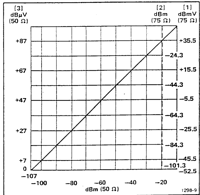
Fig. 3-11. Graph to illustrate relationship between dBm, dBmV, and dBμV (matching attenuator included where necessary).
