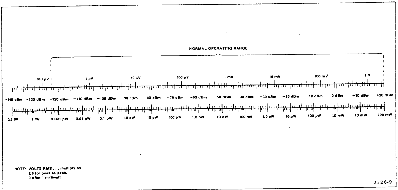
Fig. 3-9. Volts-dBm-watts conversion chart for 50 \Omega impedance.
