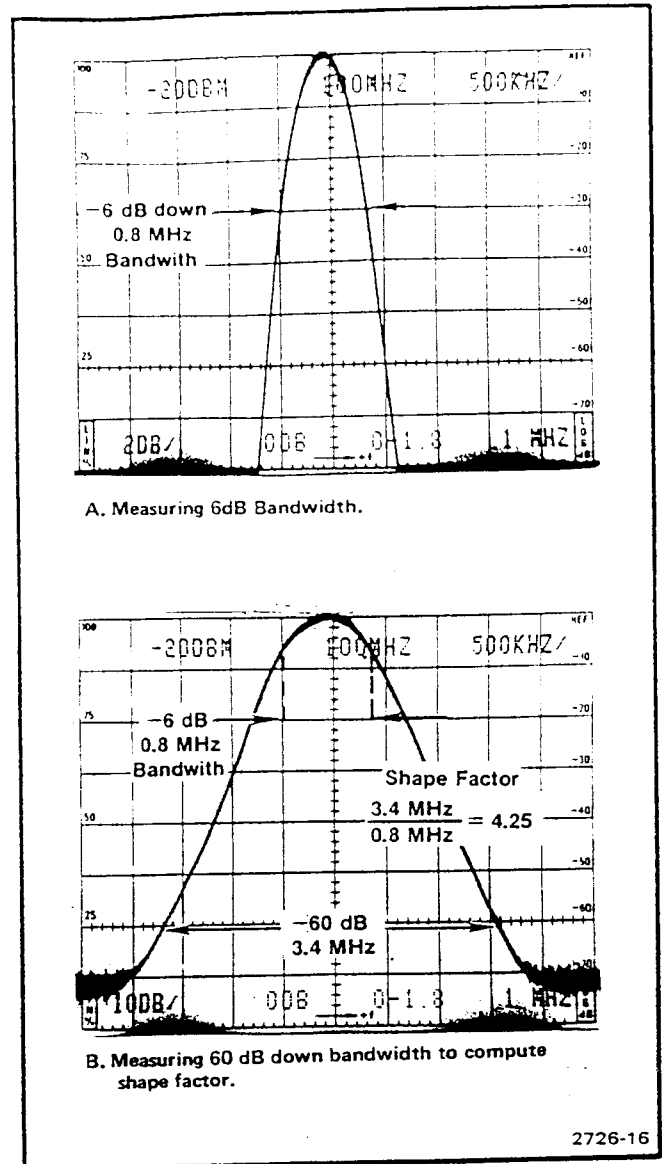
Fig. 3-5. Display to illustrate how bandwidth and shape factors are determined.
