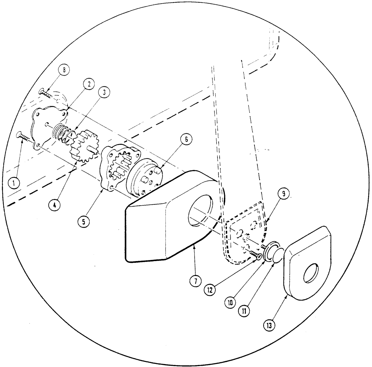
Figure 1. Partial - cabinet
