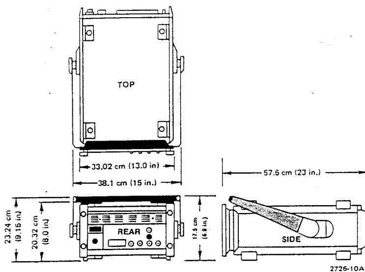
Fig. 1-1. Dimensions.
