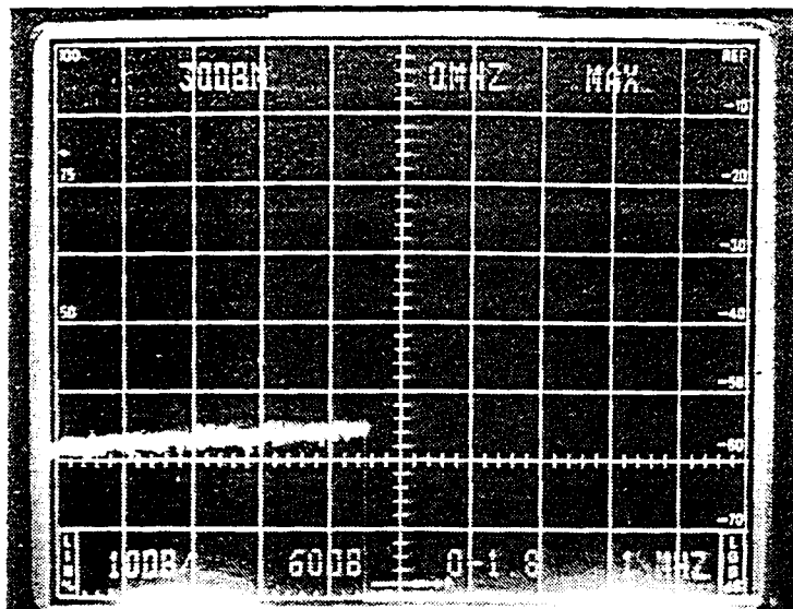
Fig. 3-3. CRT readout for power-up state (Option 1).
