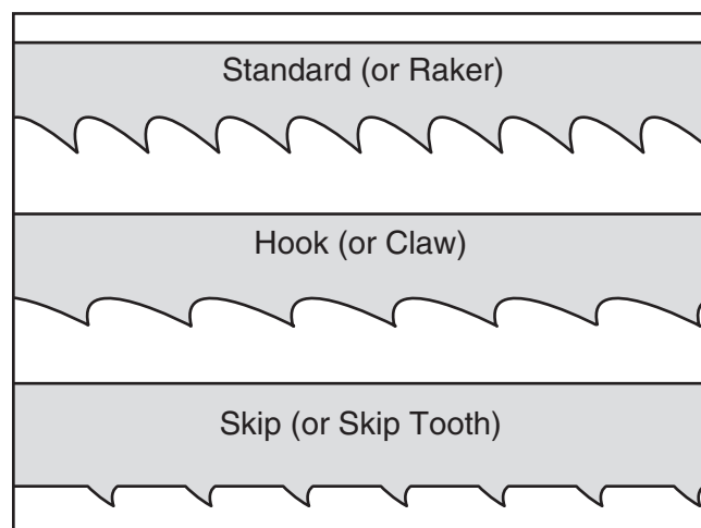
Figure 67. Typical tooth types.
