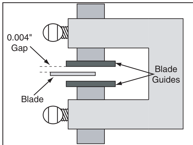
Figure 45. Correct gap between guide guides and blade.
