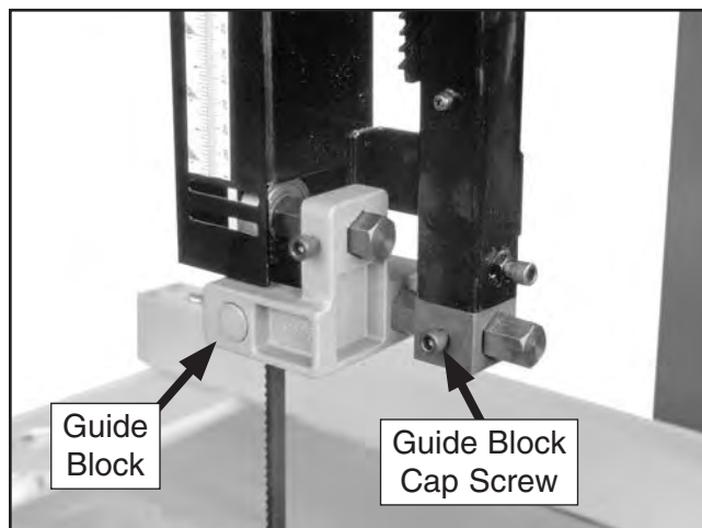
Figure 46. Back of upper blade guides.
