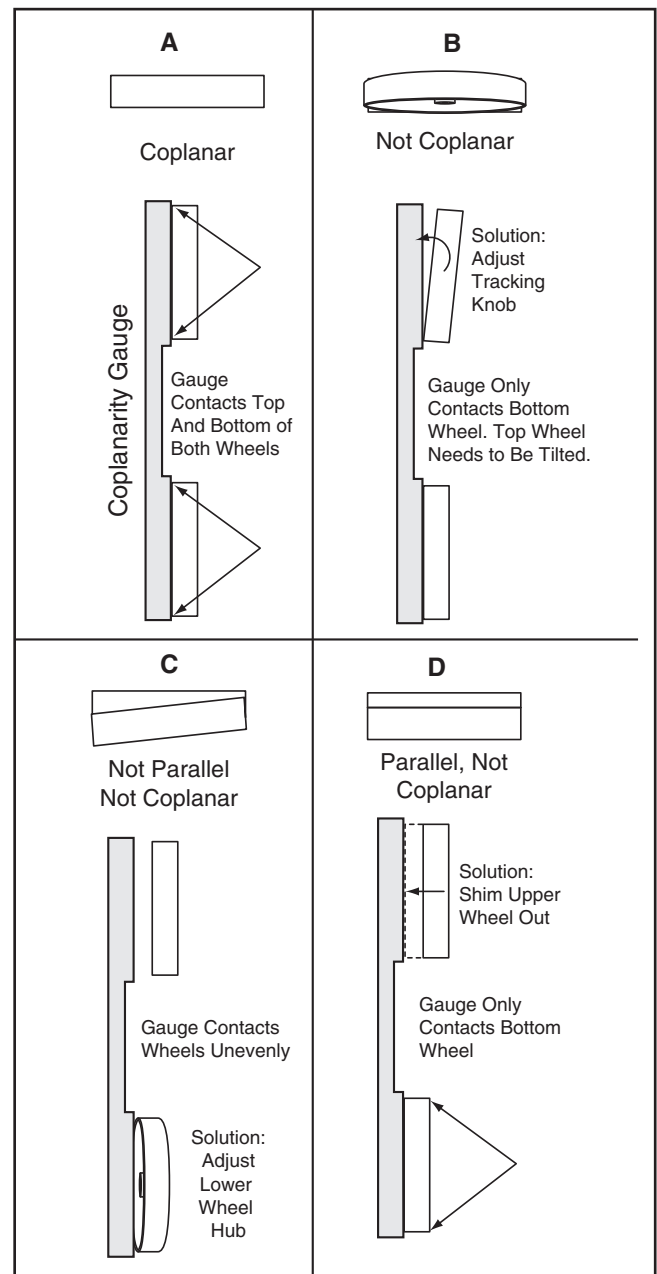
Figure 99. Coplanar diagram.
