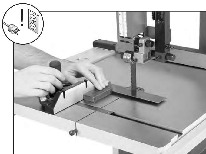
Figure 57. Squaring miter gauge to blade.
