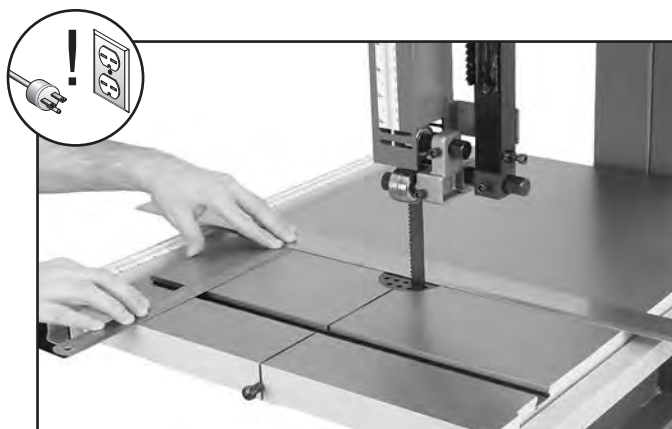
Figure 51. Measuring for miter slot to be parallel with blade.
