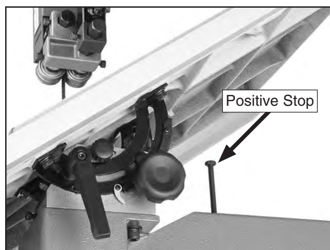
Figure 17. Positive stop bolt installed.
