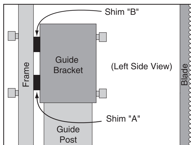
Figure 95. Location for placing shims.
