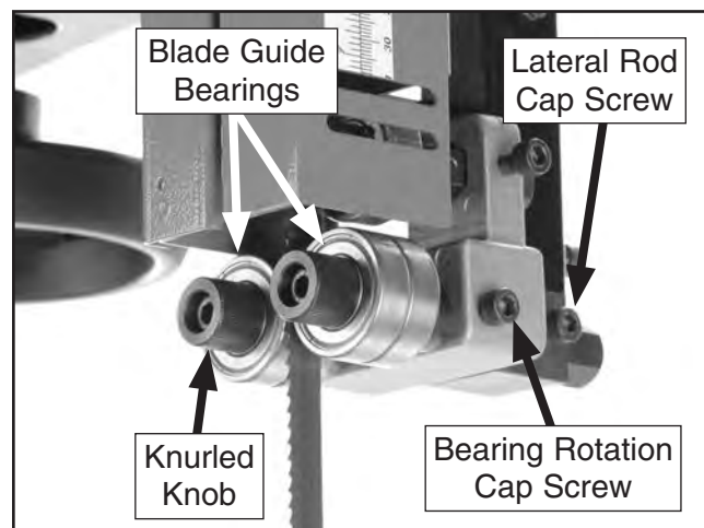
Figure 49. Blade guide controls.
