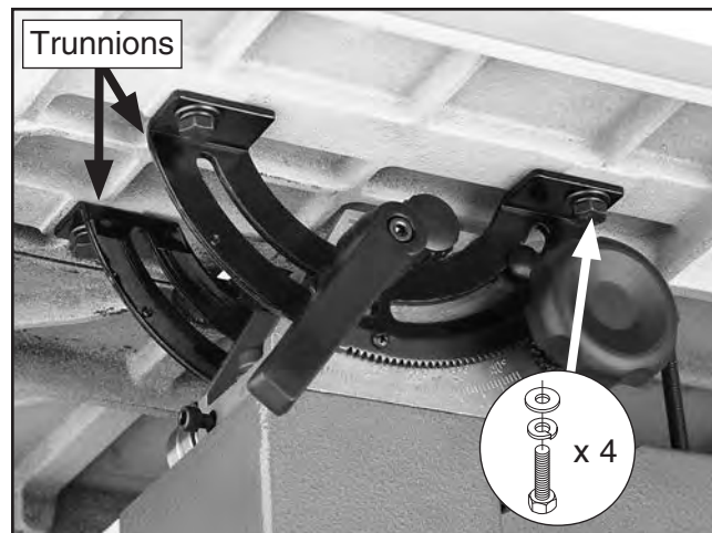
Figure 19. Mounting the table.
