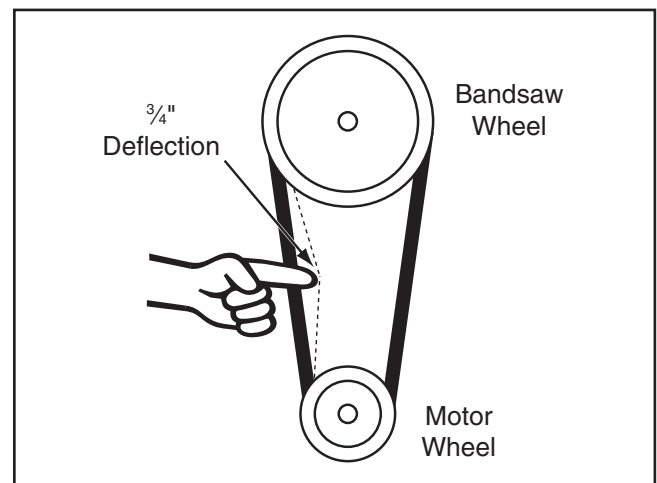
Figure 72. V-belt deflection.
