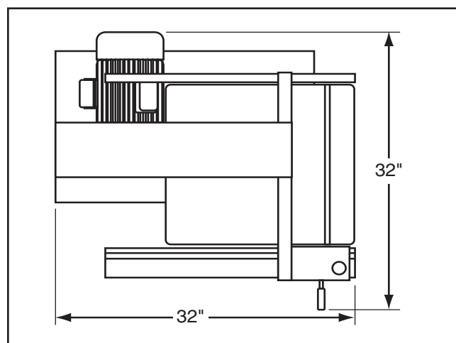
Figure 11. Minimum working clearances.
