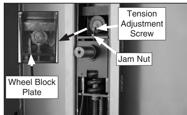
Figure 91. Example of quick-release tension lever adjustment screw.
